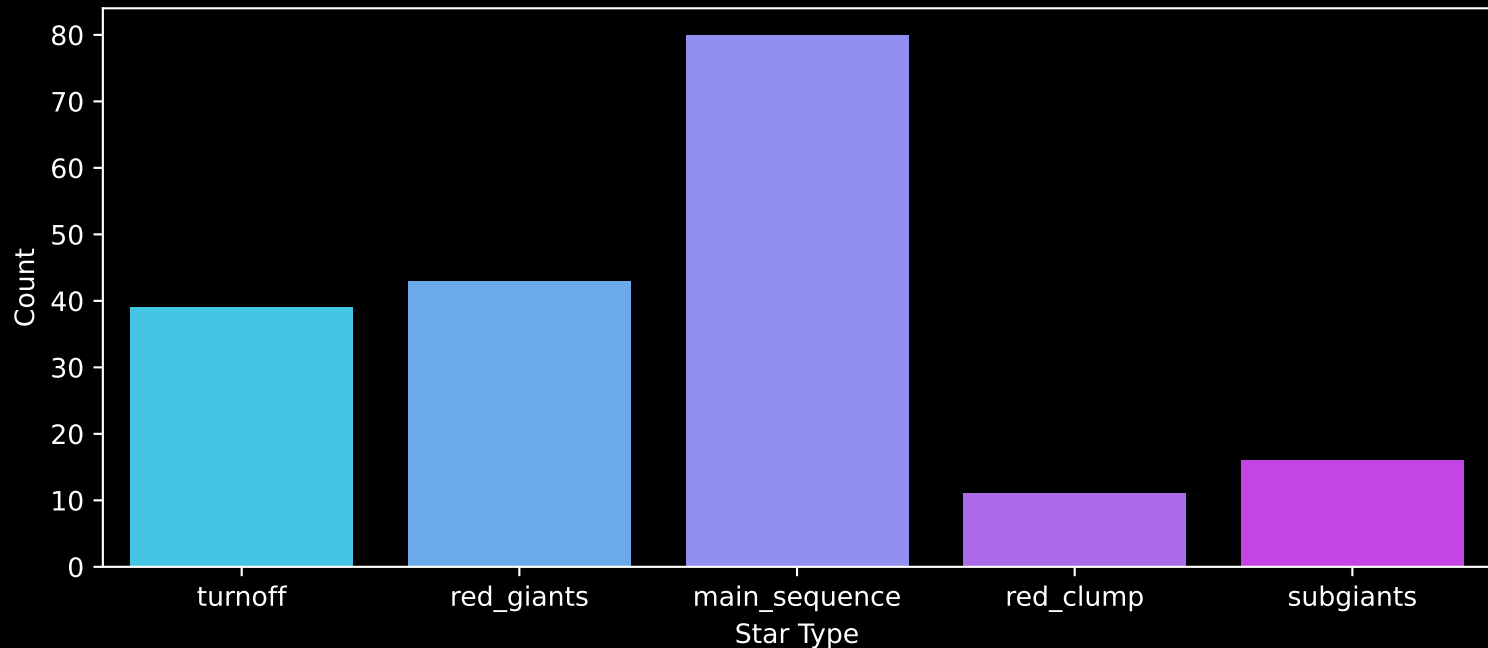
APOGEE DR17 Field: [206+29_MGA] Count plot of Star Type
