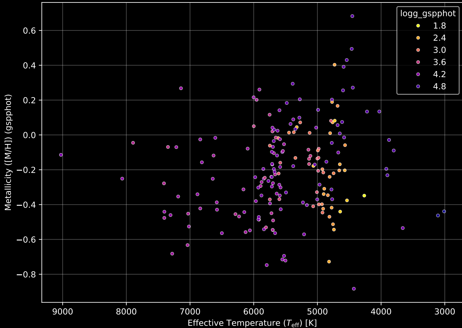
APOGEE DR17 Field: [206+29_MGA] Stellar Population Parameters (n= 189)
