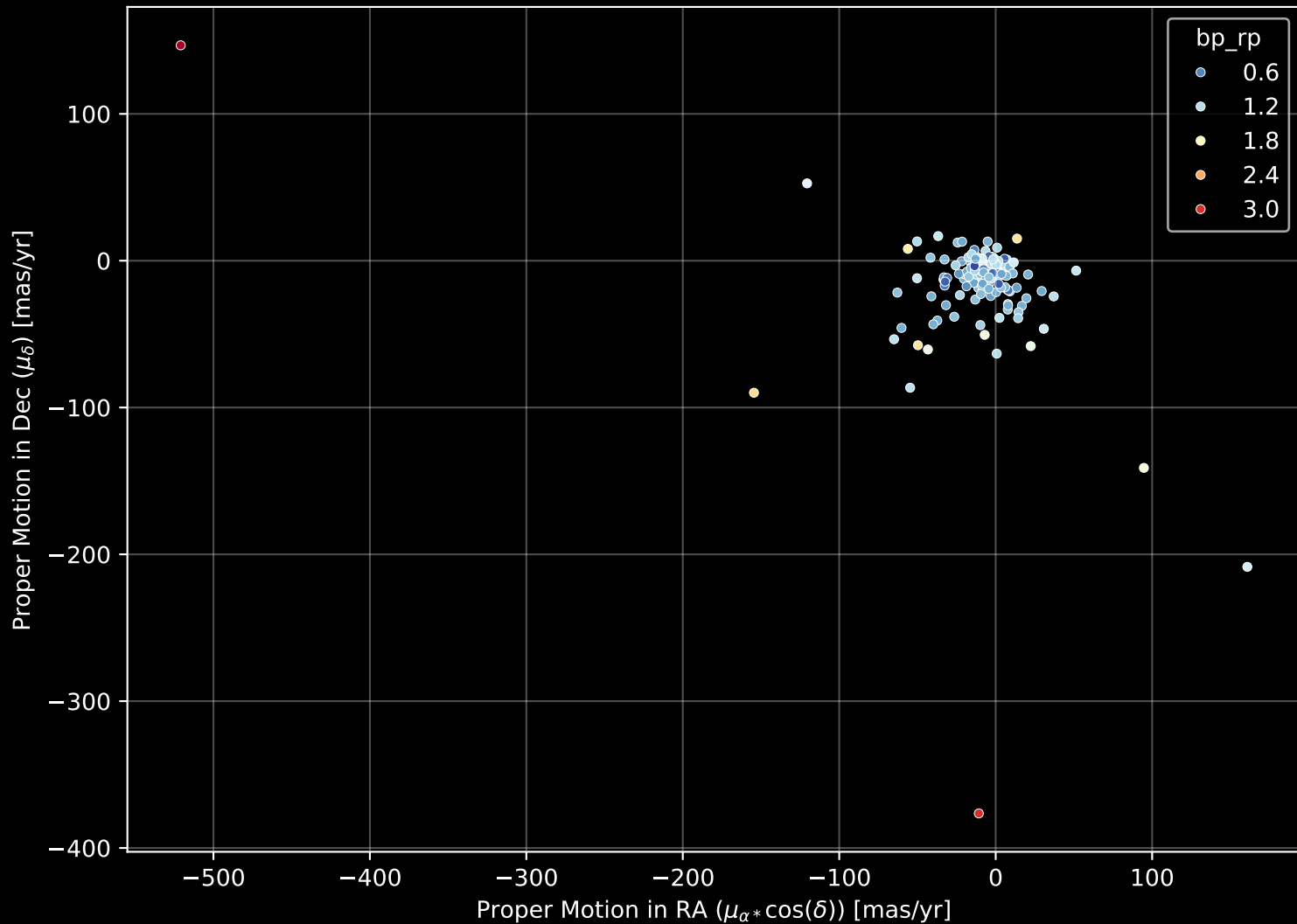
APOGEE DR17 Field: [206+29_MGA] Proper Motion Diagram (n= 189)
