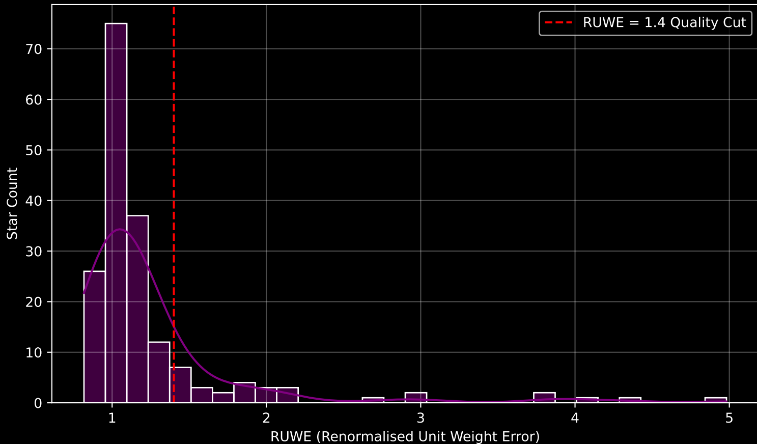
GAPOGEE DR17 Field [206+29_MGA] RUWE Distribution (n= 180)
