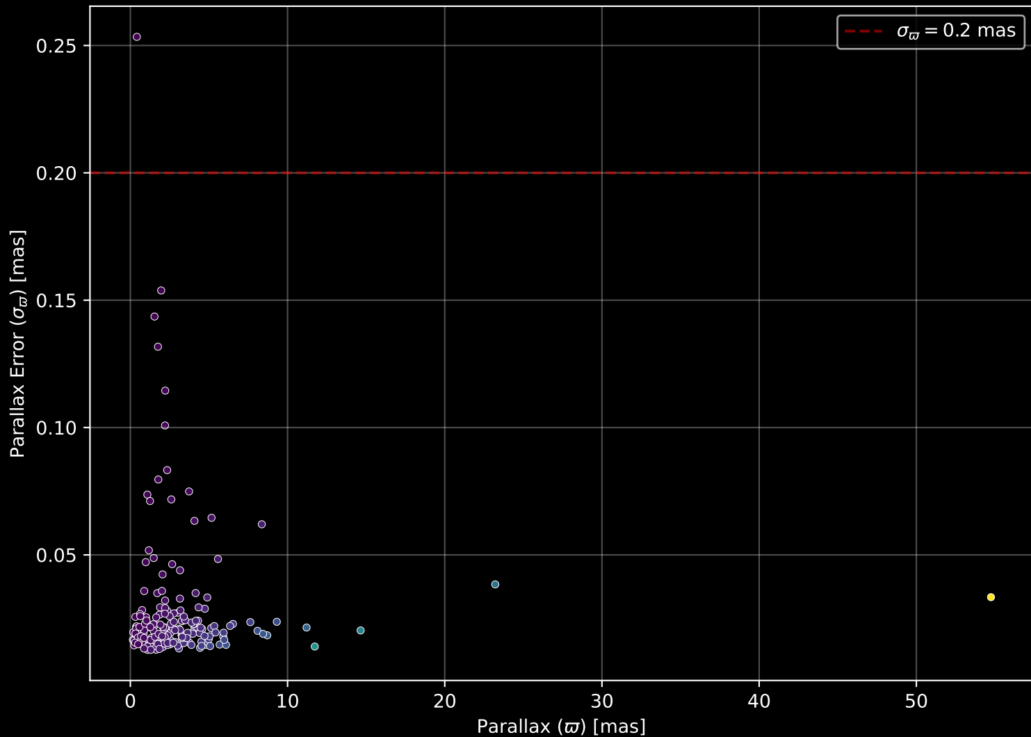
APOGEE DR17 Field: [206+29_MGA] Parallax Quality (n= 189)
