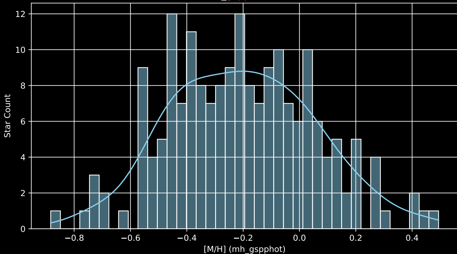
APOGEE DR17 Field: [206+29_MGA [M/H] (mh_gspphot) (n= 188)
